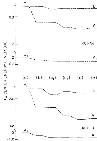
FIG. 2. Changes in the F -center energy levels due to the presence of an impurity ion in a nearest-neighbor position for the KCl:Na and KCl:Li F_A centers. The energy levels of the unperturbed F -center are shown in (a) and the changes are due to (b) the change in the ion-size correction, (c 1 ) the Stark splitting and (c 2 ) changes in the ion-size correction associated with the displacement of the impurity ion relative to the other nearest-neighbor cations, (d) the errors arising from the assumption that the F -electron wave function is constant throughout the ion core, and (e) polarization effects. The calculations were done using GA type-III and -II wave functions to represent the ground and excited states of the F electron. Each energy level is labeled with the representation of the symmetry group according to which the level transforms.
