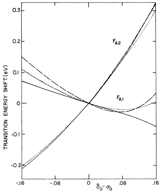
FIG. 1. Calculated shifts in the optical absorption energies of the F_{A1} and F_{A2} transition from the F -center absorption energy due to the Stark splitting associated with a radial displacement \delta_0 - \sigma_0 of the impurity ion relative to the other nearest-neighbor cations ( \delta_0 - \sigma_0 is positive for an inward displacement and has the units of the lattice constant) are shown for selected approximate forms of the F -electron wave functions in KCl. The approximate forms of the wave functions used are (a) GA type I, solid line; (b) GA type-III and type-II ground and excited state, dashed line; and (c) those given in Ref. 8, dotted line.
